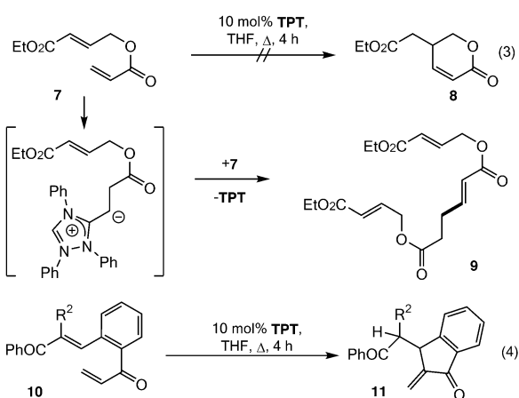
Scheme 1. Competing reactions.
