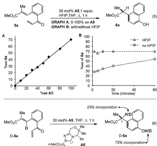
Scheme 2. Mechanistic studies.
