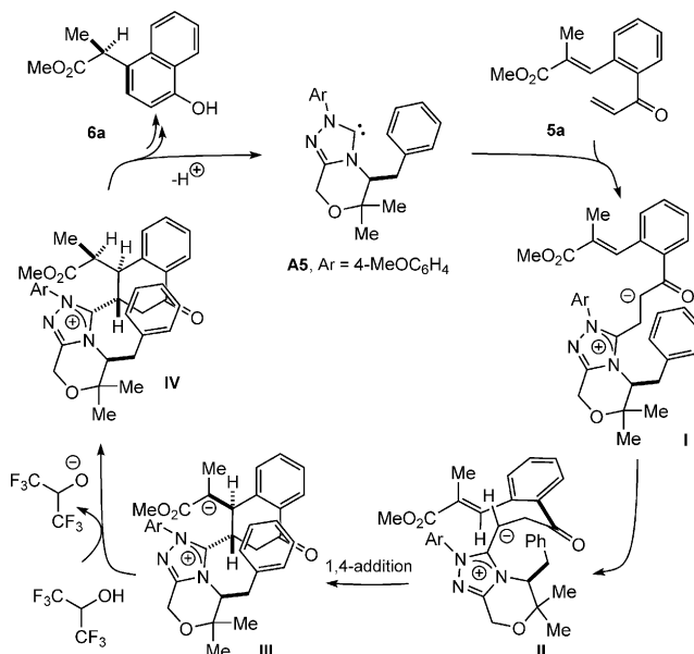
Scheme 3. Plausible mechanism.
